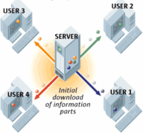
Source: BitTorrent
